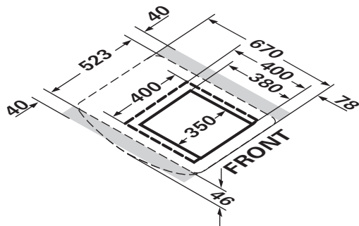
Figure 11 – Air distributor
